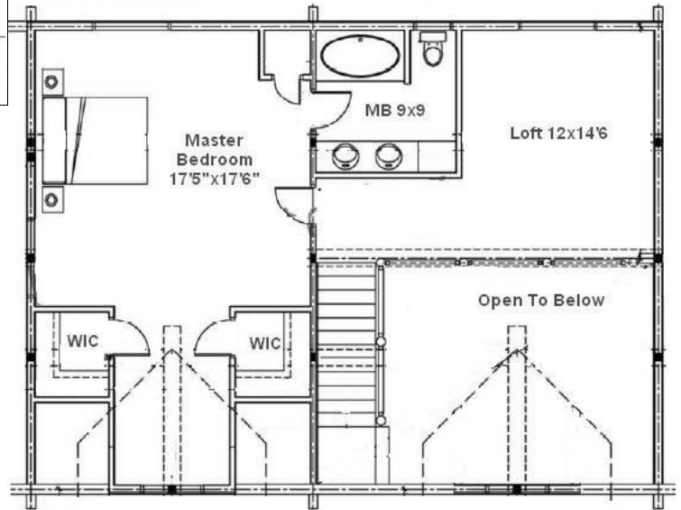
Second Floor 858 Sq. Ft.
