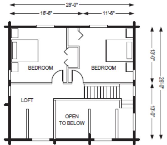
Second Floor 518 sq. ft.
