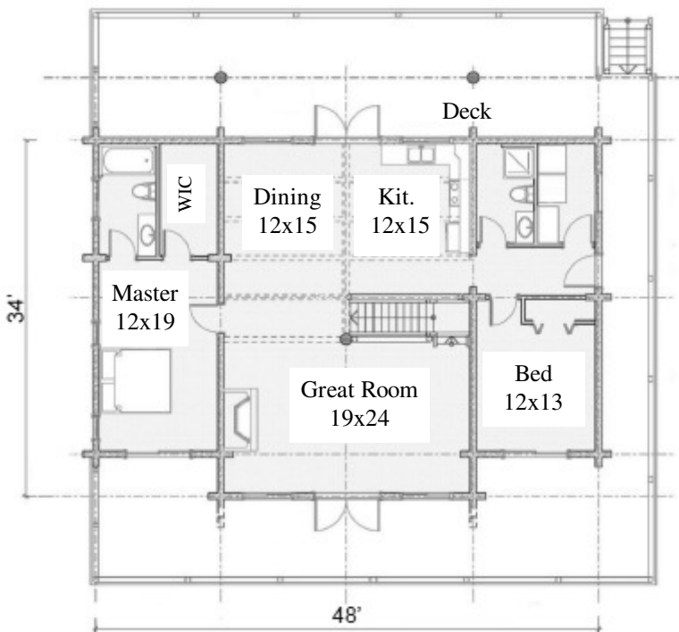
Main Floor 1,536
