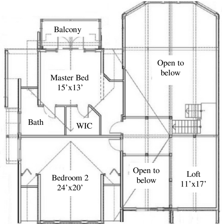
Second Floor 1,000 sq. ft.
