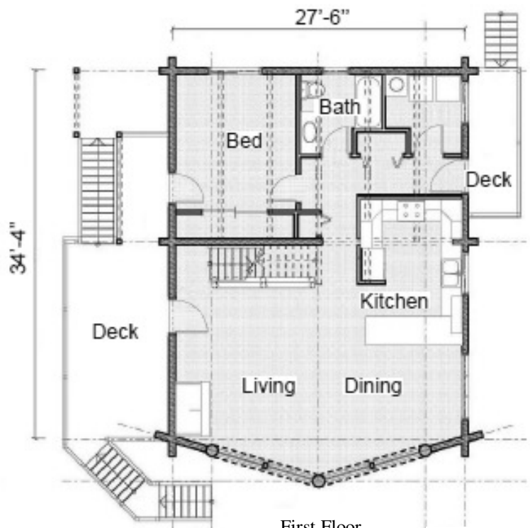
First Floor 1,000 sq. ft.
